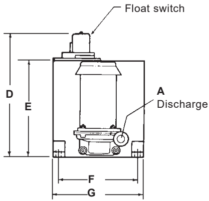
End view steel 10 gallon Simplex unit
