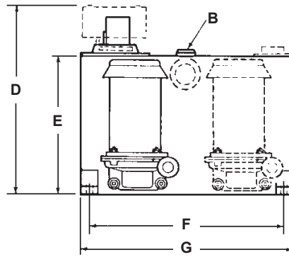
End view steel 20 gallon Simplex and duplex unit
