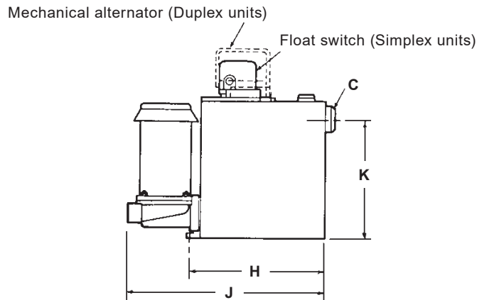
Side view steel 10 and 20 gallon Simplex and duplex unit
