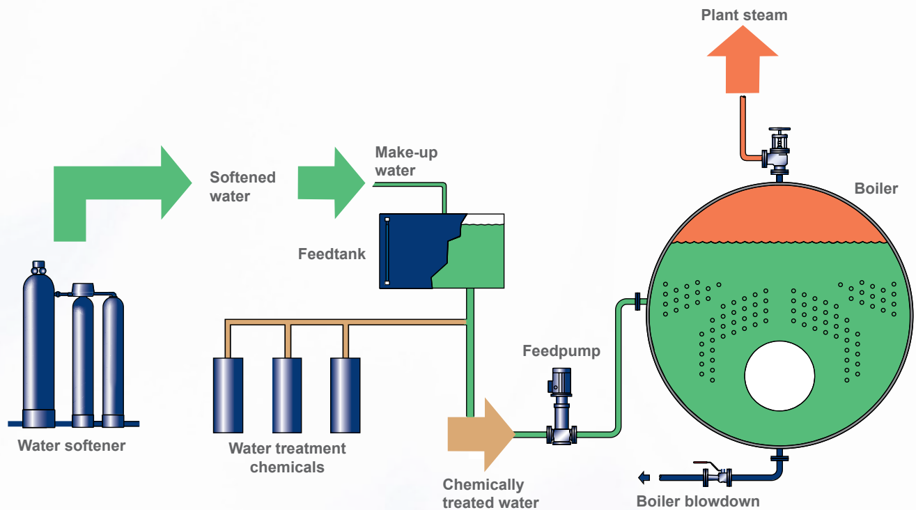
Figure 2: Plant steam generation
