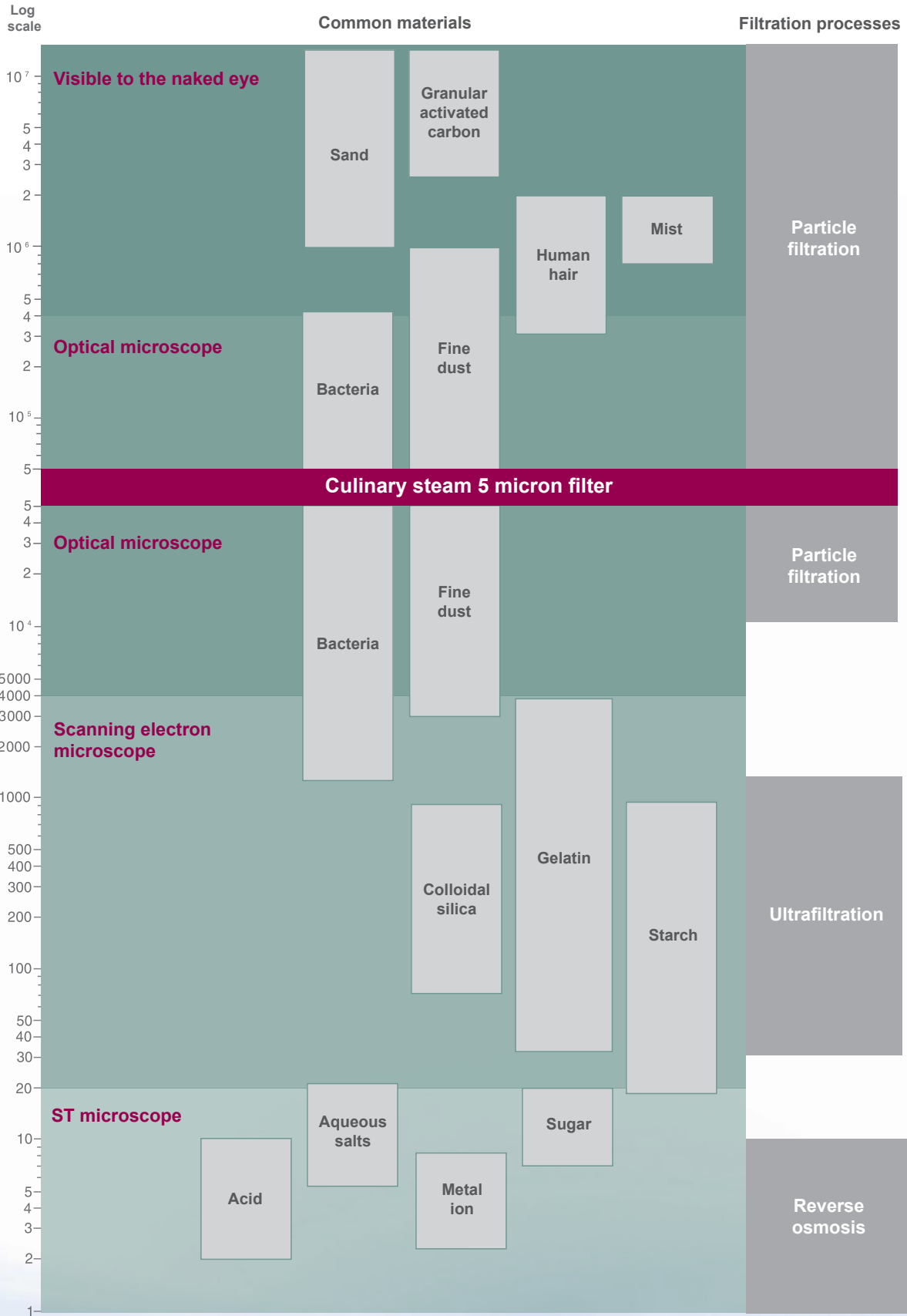
Figure 5: Filtration spectrum
