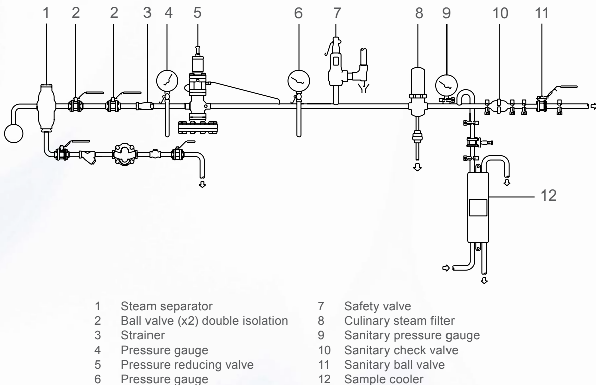
Figure 4: Typical filtered steam station
