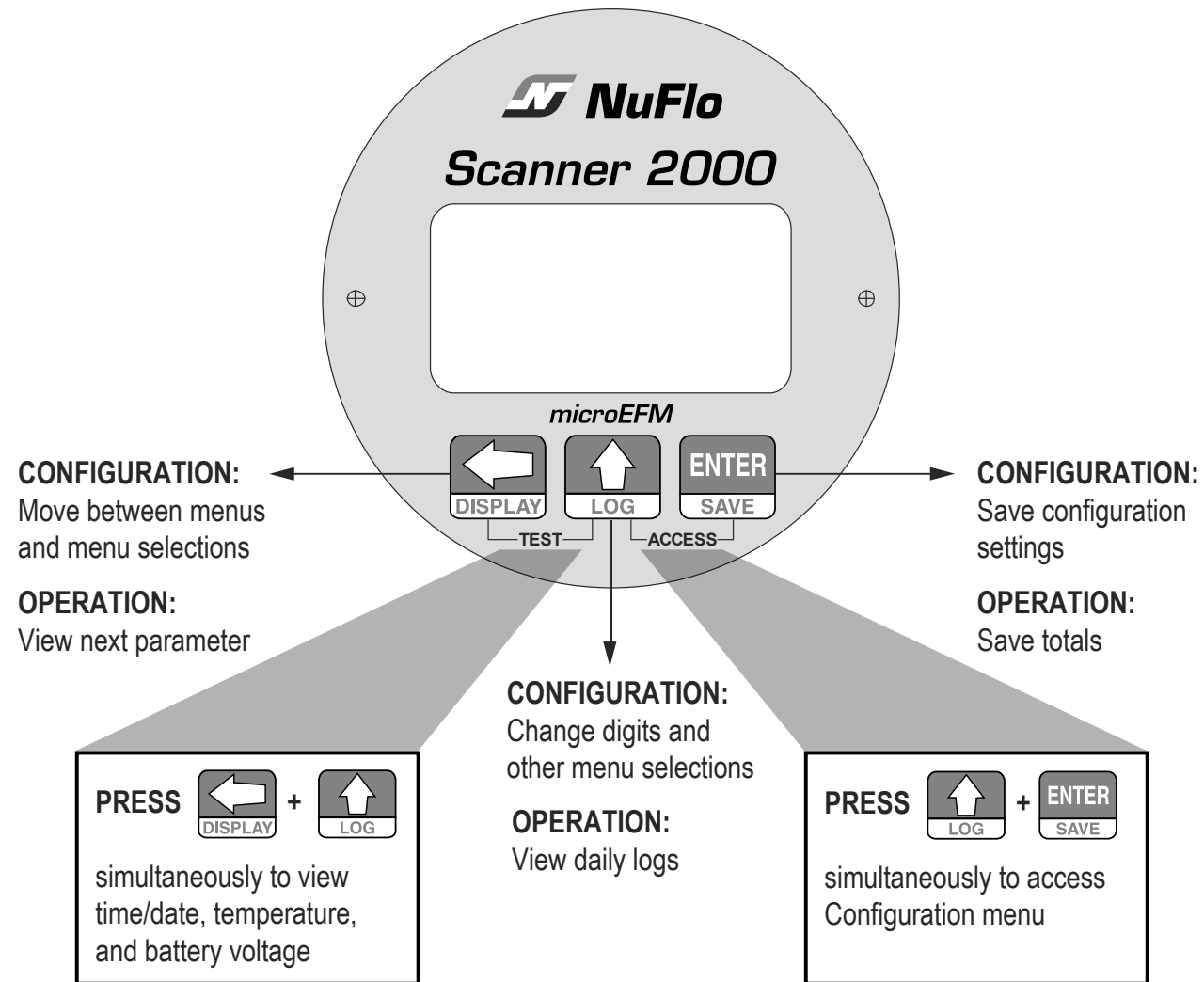
Figure 1.7—Keypad functions
