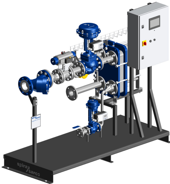
EasiHeat Dual Control System
