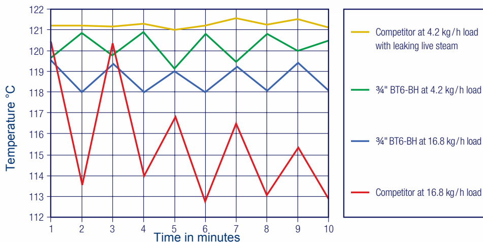
Temperature control @ nominal 1 barg
