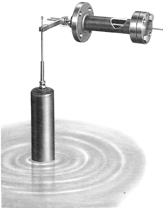
Fig. 4 - Displacer and torque tube unit.
