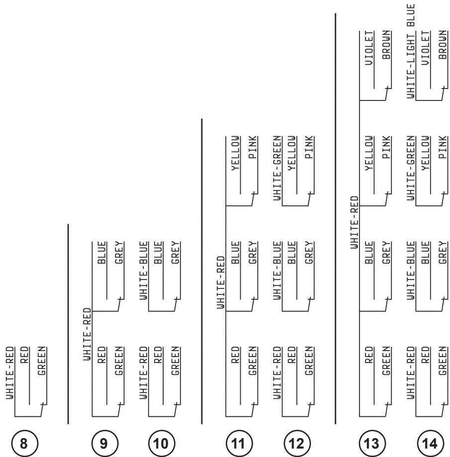
Identification numbers wiring diagrams
