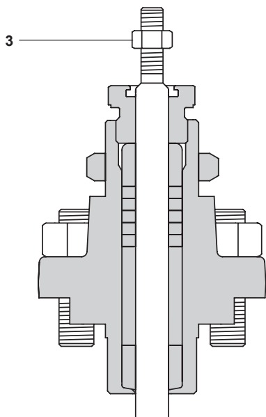
KEA valve with PTFE packing
