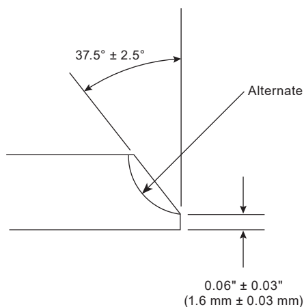
Fig. 3 Weld bevel details for GTAW root pass (wall thickness over 0.12" (3 mm) to 0.38" (10 mm) inclusive)
