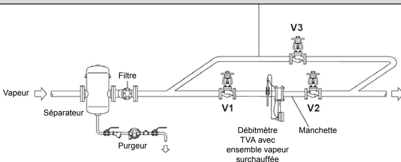
Fig. 5 - Installation type
