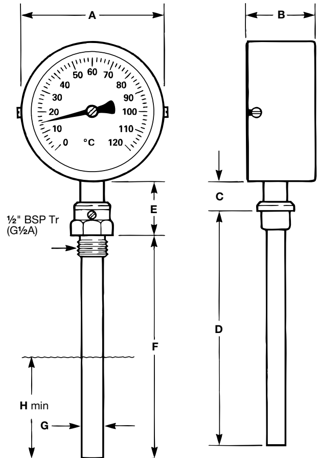
Thermometer (Aluminium body) with pocket
