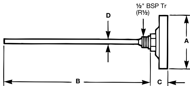
Thermometer (Austenitic stainless steel body)
