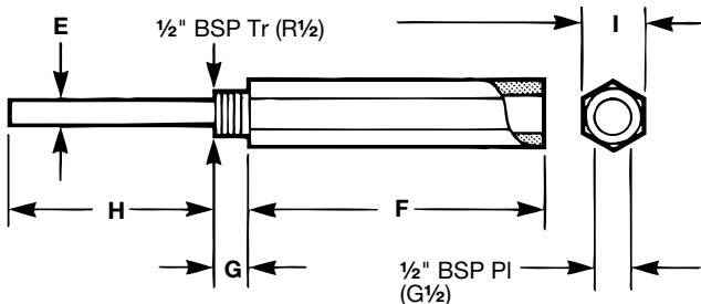
Optional pocket (Stainless steel)
