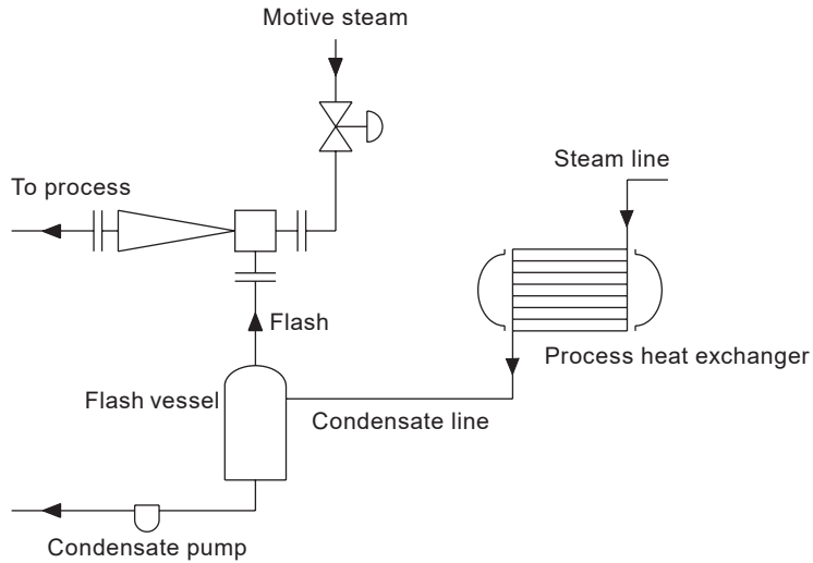
Typical SJT Steam Jet Thermocompressor application
