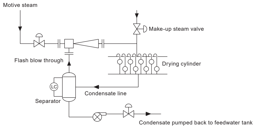
Typical Paper Mill application
