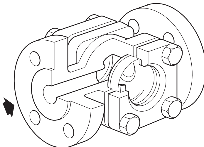
DN32 shown having an integral flange Please note that flanges are welded onto the body of the smaller DN15 to DN25 units.
