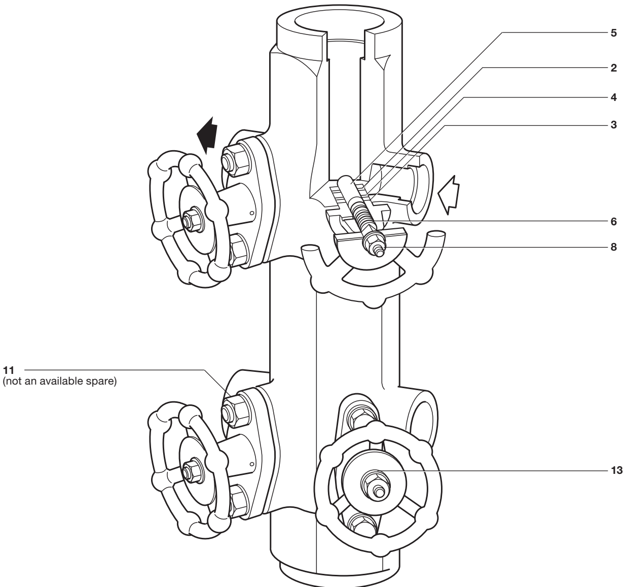
MSC04 shown having socket weld connections
