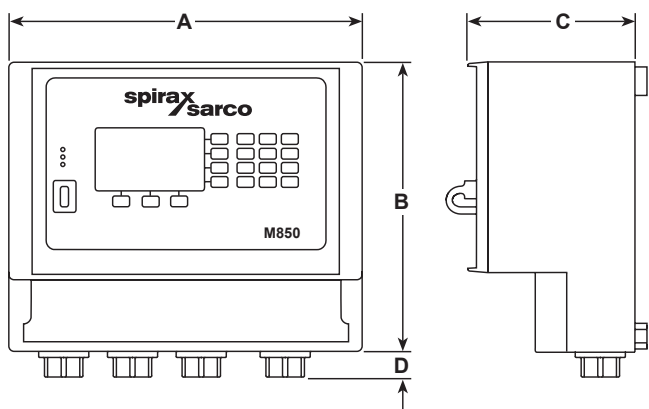
M850-W-x-UL version
