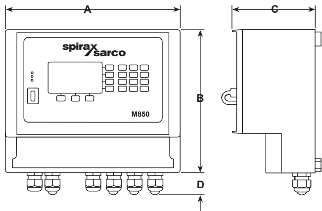
M850-W-x (wall mounted)
