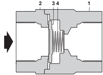
Standard DCV41 with metal seat
