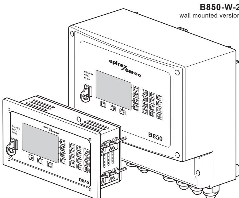
B850-P-2 panel mounted version
