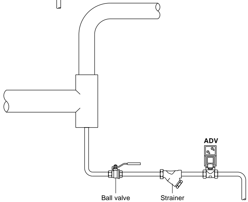
Fig. 2 Draining a compressed air main relay point
