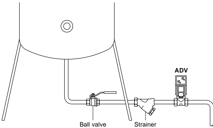
Fig. 1 Draining a receiver or large filter
