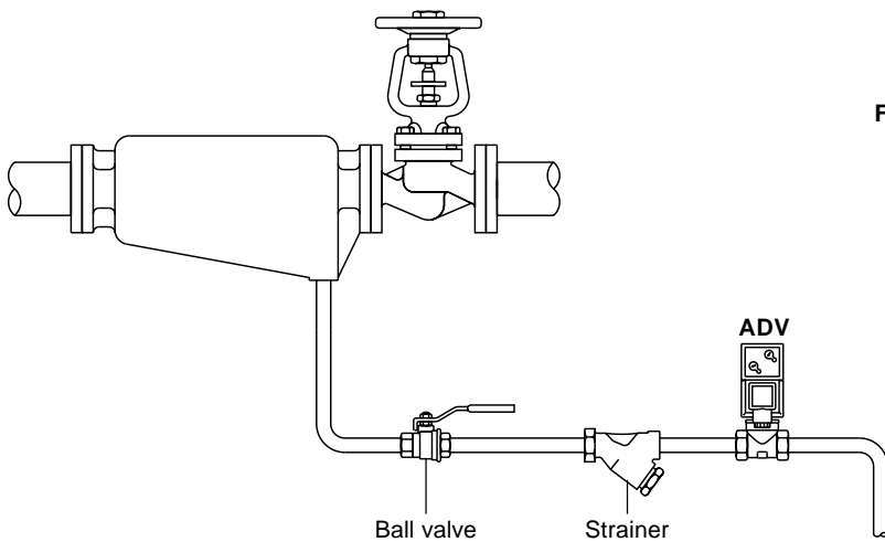
Fig. 3 Draining a separator on a compressed air main
