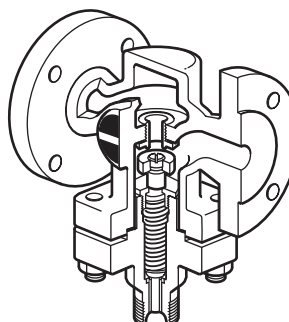
KA31 (DN32 - DN50 screwed) KA33 (DN32 - DN50 flanged) KA43 (DN15 - DN50 flanged)
