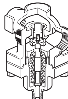
KB31 (DN32 - DN50 screwed)* KB51 (DN32 - DN50 screwed)* KC51 (DN40 - DN50 screwed)
