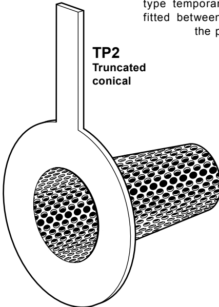
Fig. 1 TP1, TP2 and TP3 temporary cone and flat shaped strainers and spacer ring
