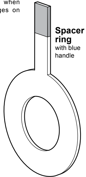
Fig. 1 TP1, TP2 and TP3 temporary cone and flat shaped strainers and spacer ring
