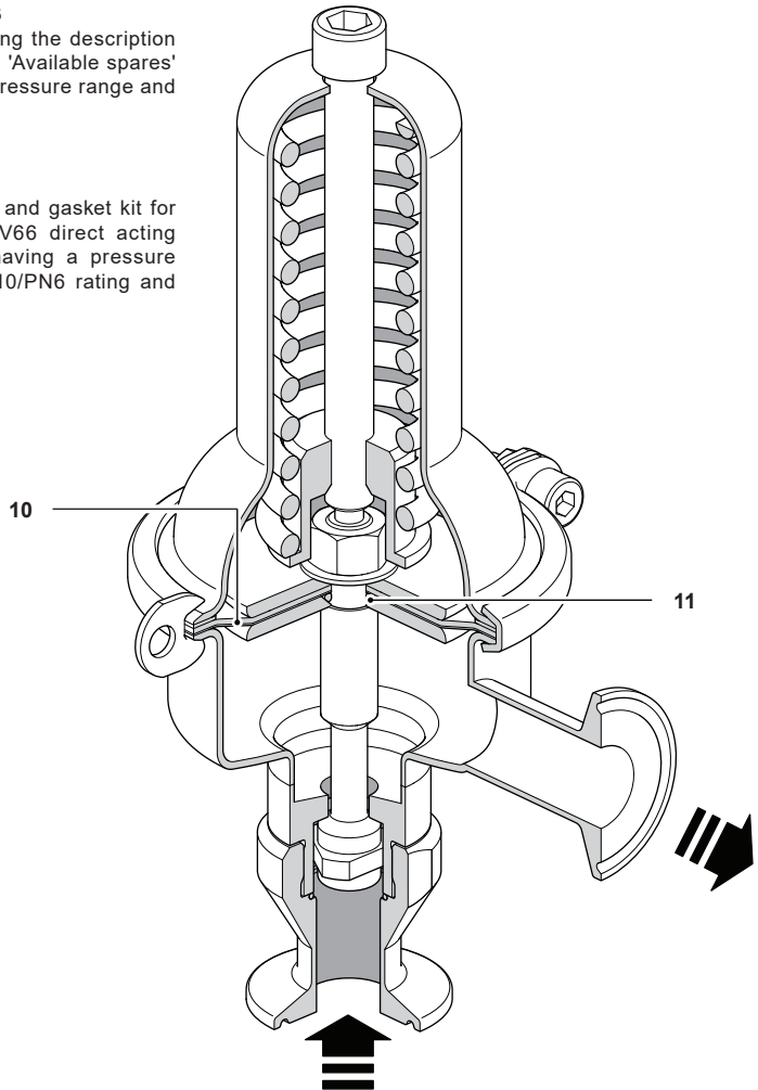
Fig. 7 SRV66 spares
