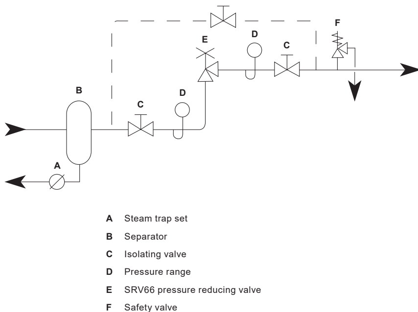
Fig. 2 Recommended installation
