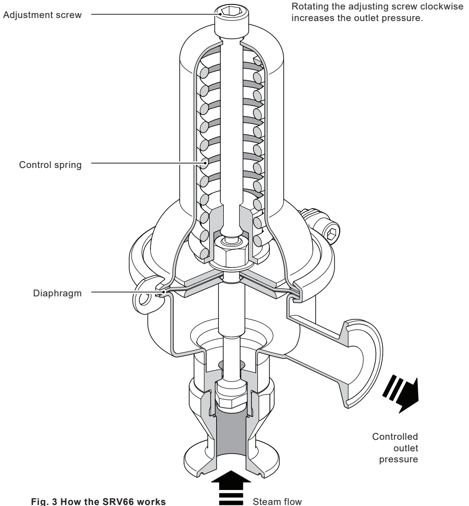
Fig. 3 How the SRV66 works
