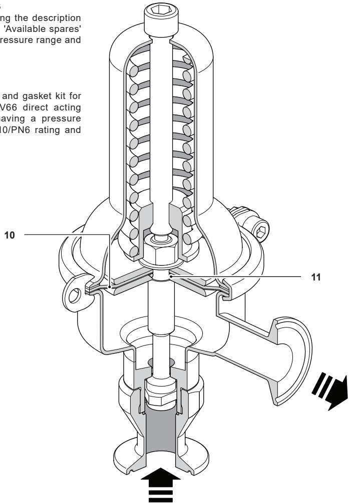
Fig. 7 SRV66 spares
