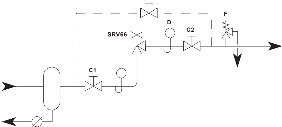
Fig. 4 SRV66 - Commissioning
