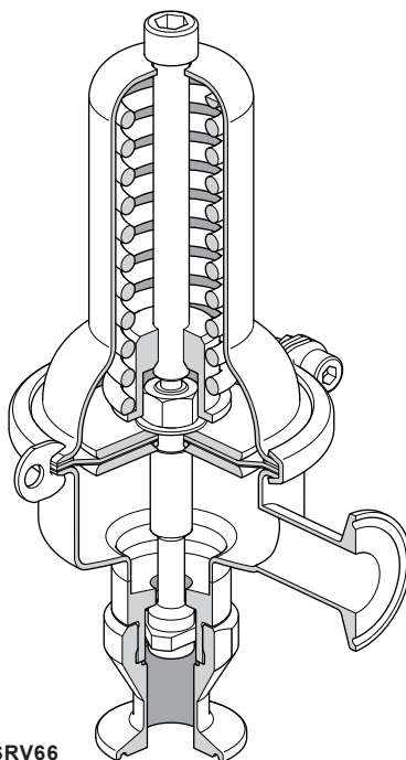
Fig. 1 SRV66
