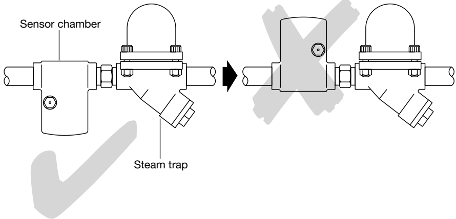
Fig. 2 Correct installation
