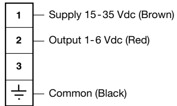
Fig. 8 Medium sensitivity (Up to 1050 mm (41") immersed length) No link
