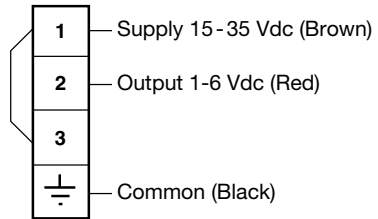
Fig. 7 High sensitivity (Up to 500 mm (20") immersed length) Link 1 + 3 (Including all probes up to 550 mm length)
