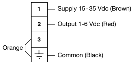
Fig. 9 Low sensitivity (Longer immersed lengths) Link 3 + Earth
