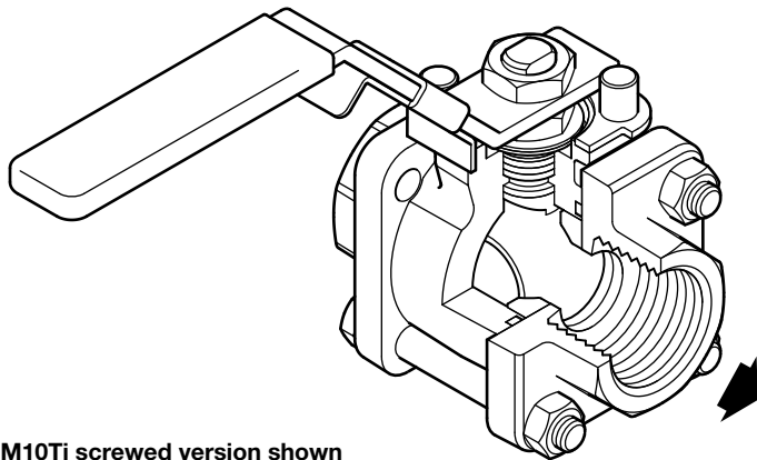
Fig. 1 M10Ti screwed version shown
