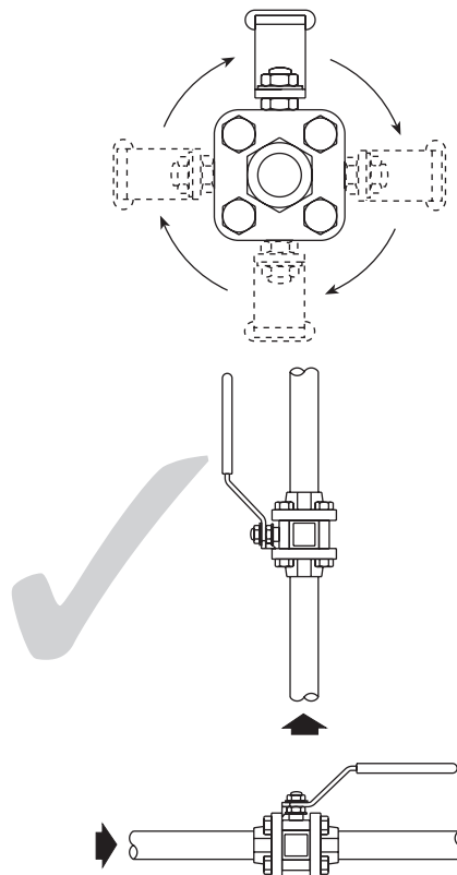
Fig. 2 Correct installation for gas service
