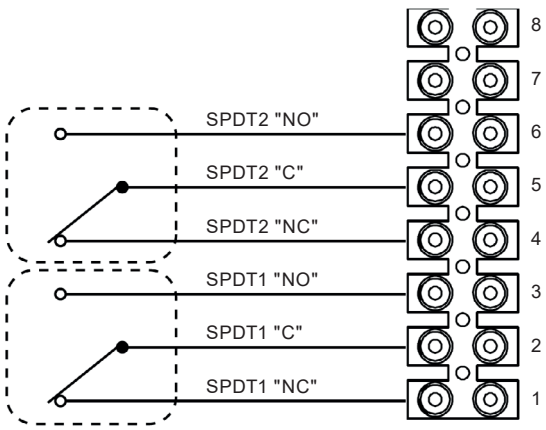
Fig. 4 LSB71 (for other sensors contact Spirax Sarco)
