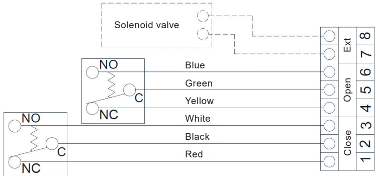
Fig. 3 LSB31 (for other sensors contact Spirax Sarco)
