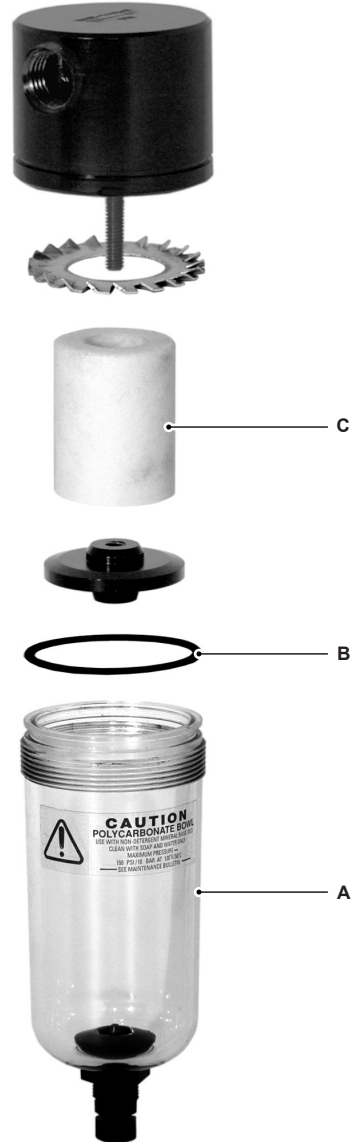
Fig. 3 Spare parts
