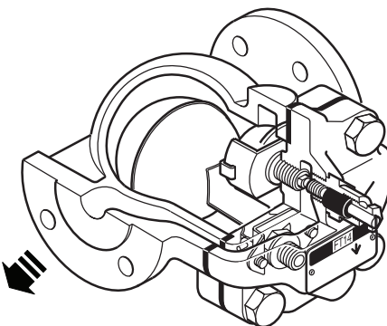
Fig. 4 FT14-C (R-L) flanged
