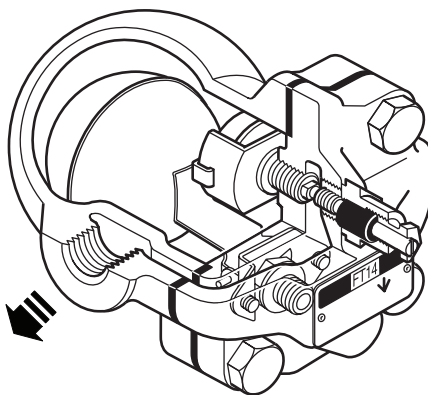
Fig. 2 FT14-C (R-L) screwed
