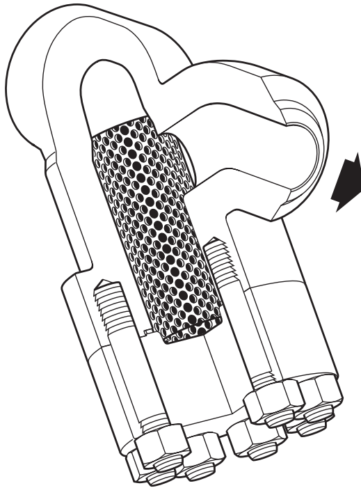
Fig. 1 Fig 18HP, alloy steel, butt weld, Y-type strainer with flanged screen cover
