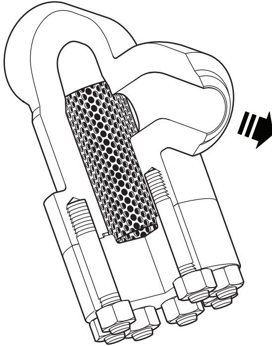
Fig. 1 Fig 18HP, alloy steel, butt weld, Y-type strainer with flanged screen cover
