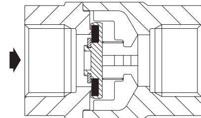
Fig. 2 Soft seat option (for screwed version only)
