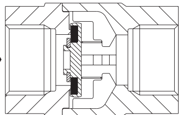
Fig. 2 Soft seat option (for screwed version only)
