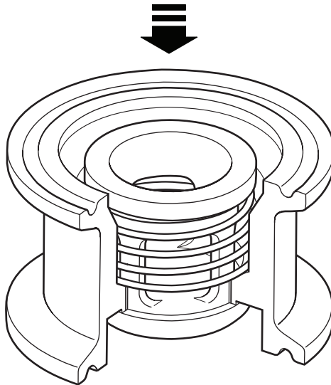
Fig. 1 CVS10 with metal seat and sanitary clamp
