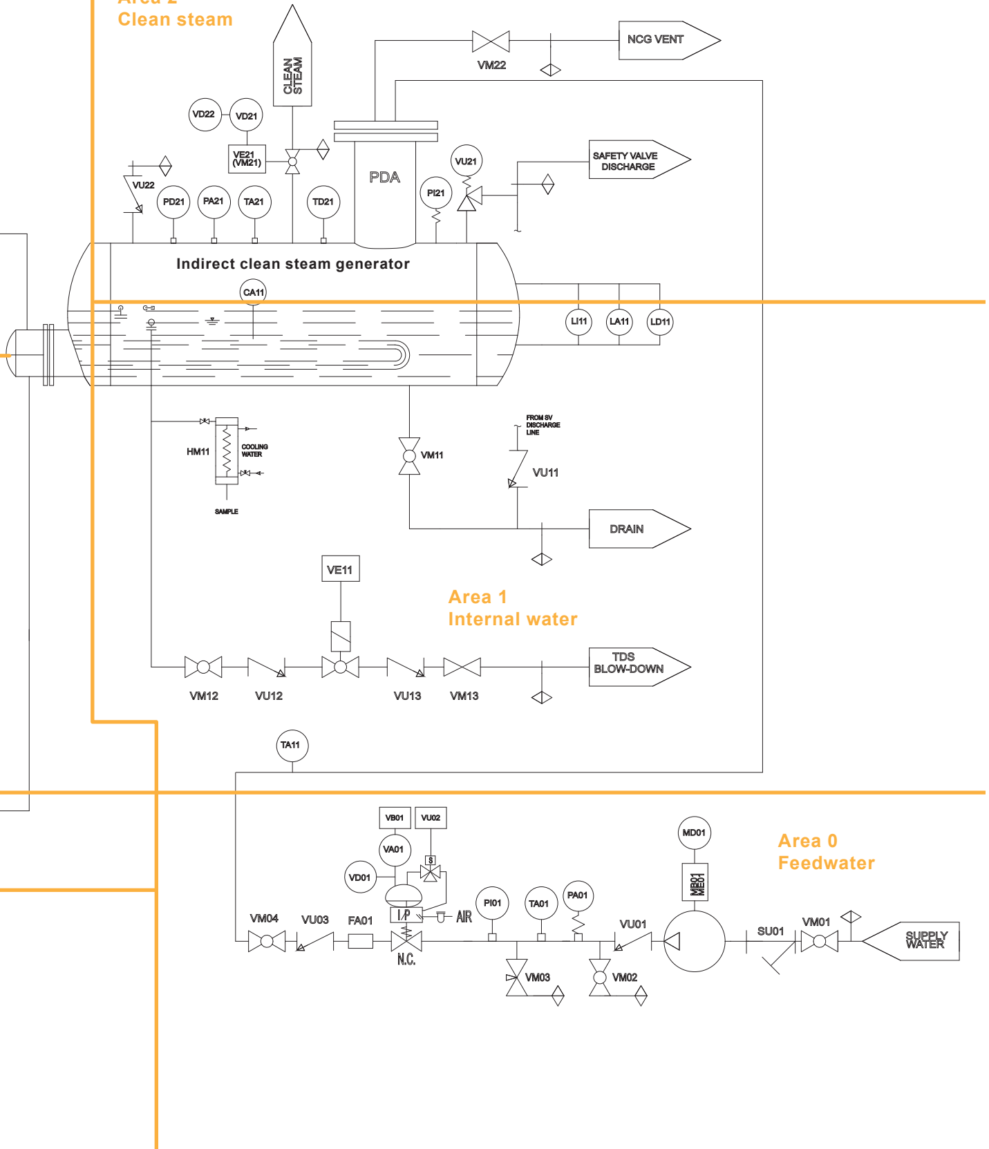
CSG-HS Clean Steam Generation System
