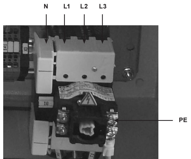
Fig. 8 Version with three-phase + N power supply
