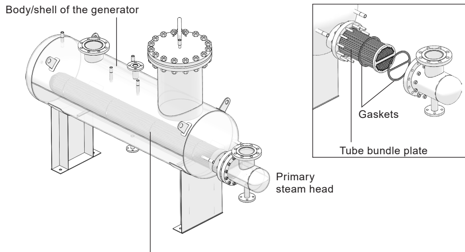
Fig. 9 "U" shaped tube bundle
