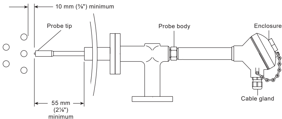
Fig. 2 Installation diagram
