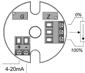
Converter for safe zone
