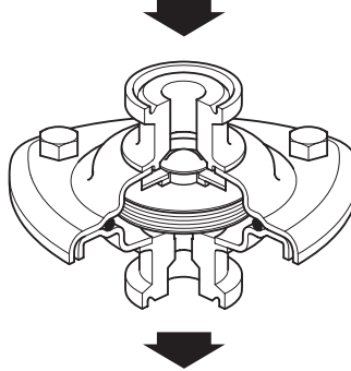
Fig. 2 BTM7 with sanitary clamp compatible hygienic connections
