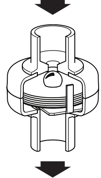
Fig. 3 BTS7 with butt weld ends
