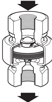
Fig. 4 BTS7 with screwed connection
