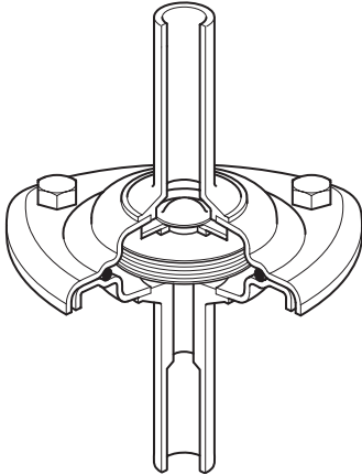
Fig. 1 BTM7 with butt weld ends
