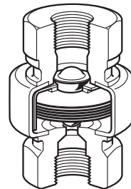
Fig. 4 BTS7 with screwed connection
