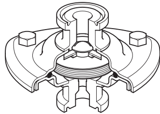
Fig.2 BTM7 with sanitary clamp compatible hygienic connections
