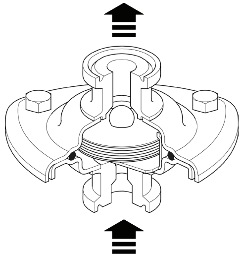
Fig. 1b Sanitary clamp ended variant
