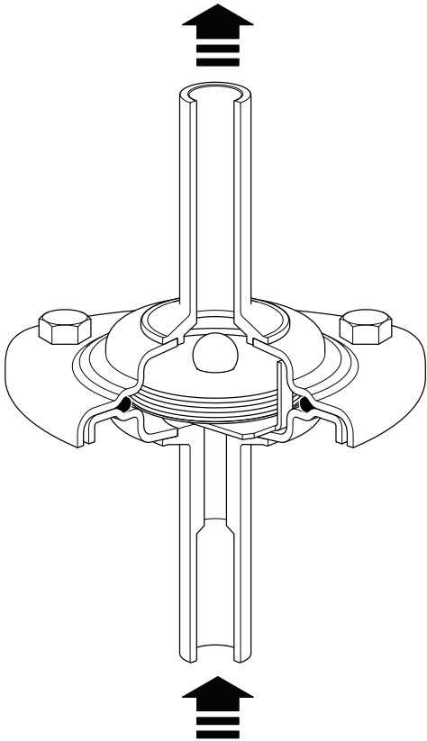
Fig. 1a Tube ended variant
