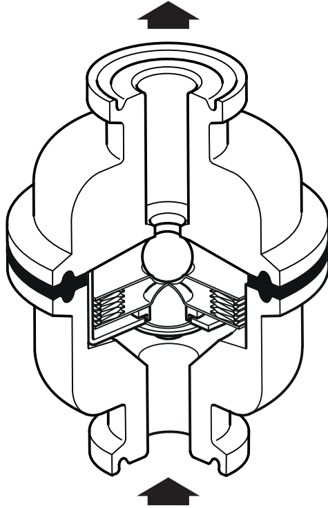
Fig. 1 AVM6.1 (clamp removed for clarity)
