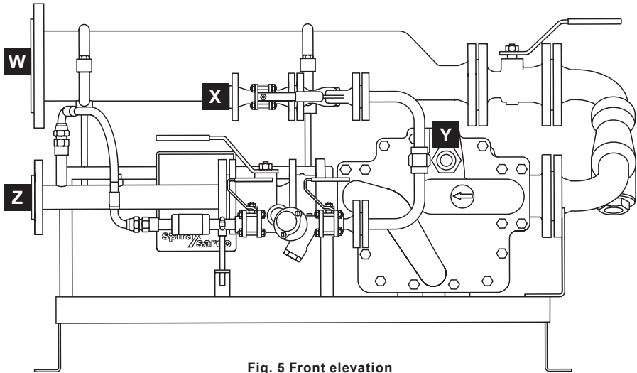
Fig. 5 Front elevation
