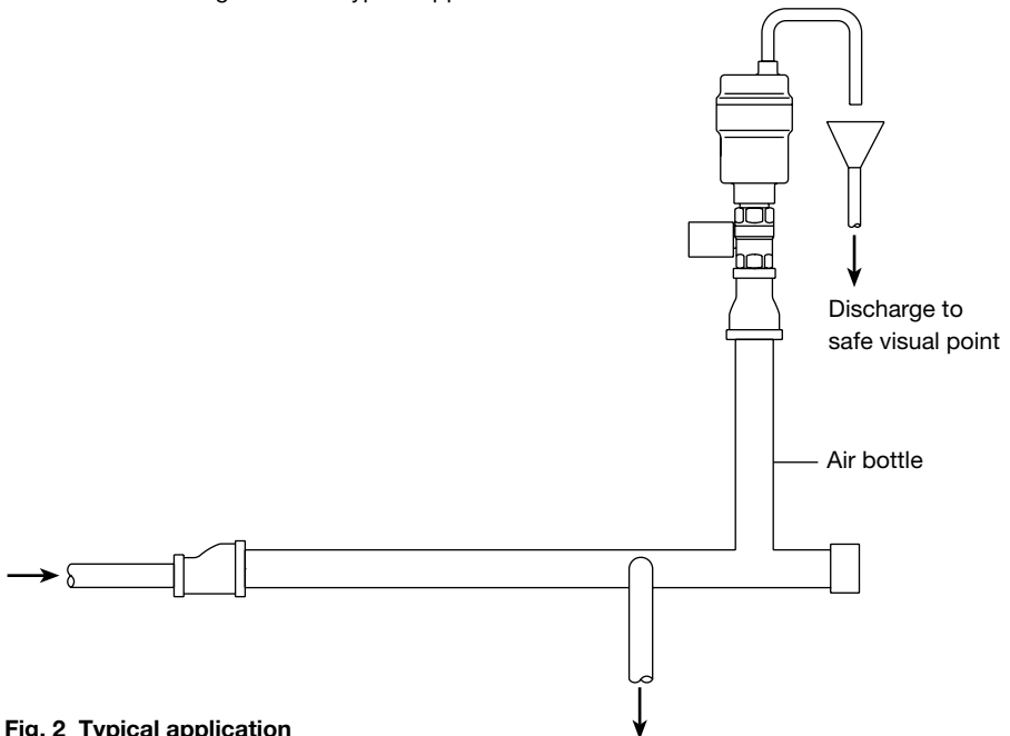
Fig. 2 Typical application
