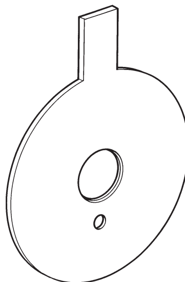
M410 orifice plate
