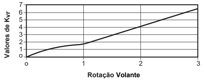
BSAT - DN20 (3/4")
