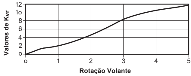
BSAT - DN25 (1")
