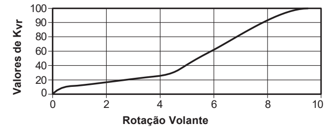
BSAT - DN80 (3")
