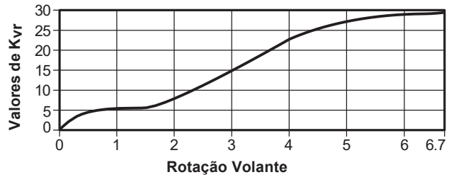
BSAT - DN40 (1 1/2")
