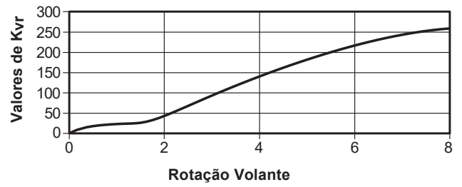
BSAT - DN125 (5")
